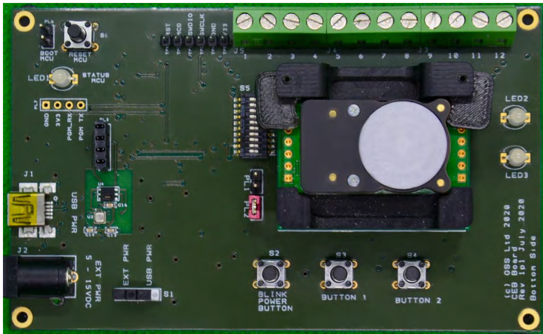
Figure 2: Top Side Evaluation Board
